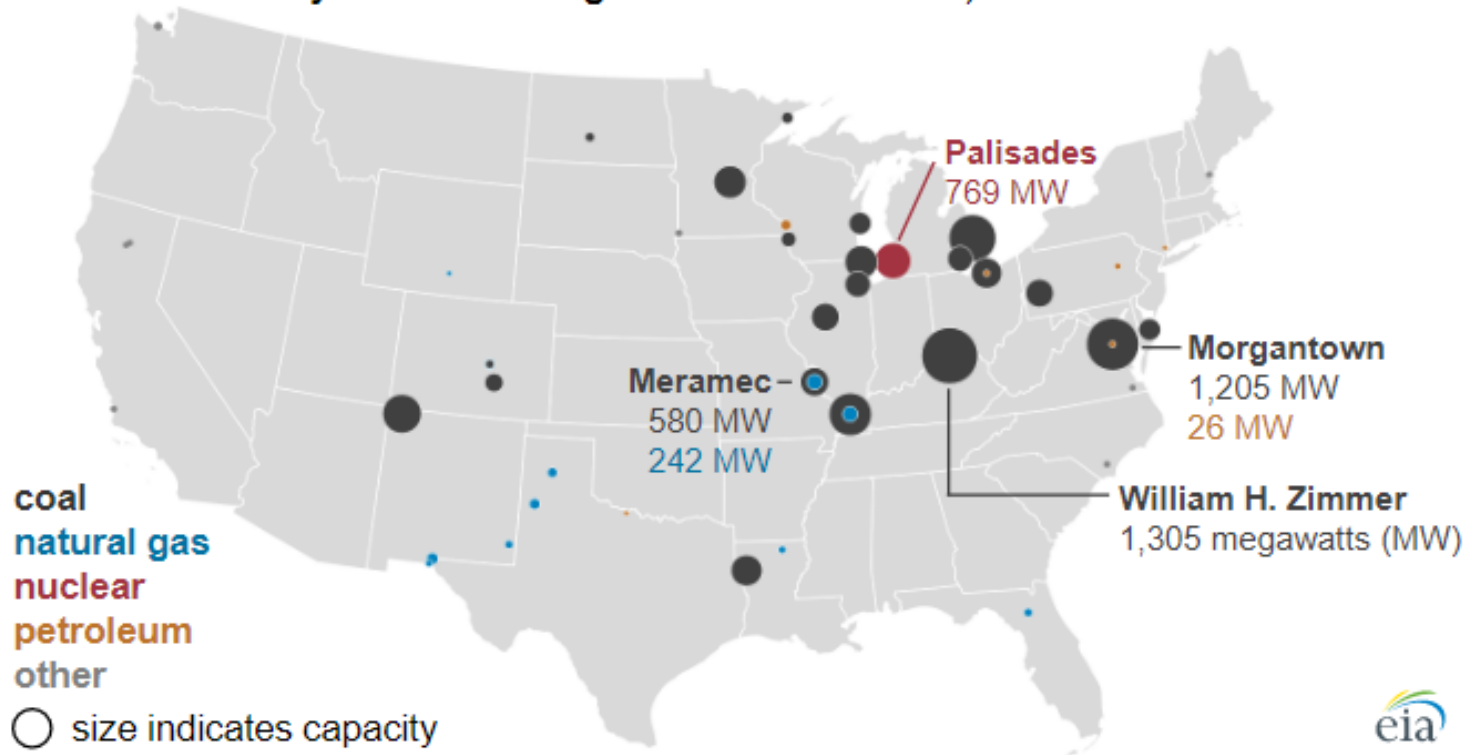
Planned U.S. utility-scale electric generator retirements, 2022
